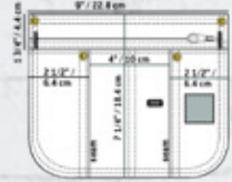
CHEST POCKET
